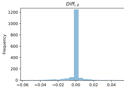
(a) Histogram of Diff_i .
