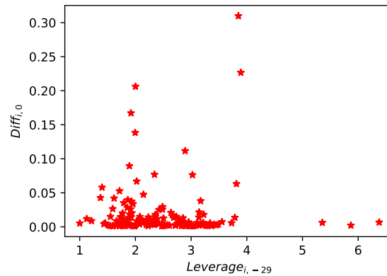
(b) Leverage vs Diff_i .
