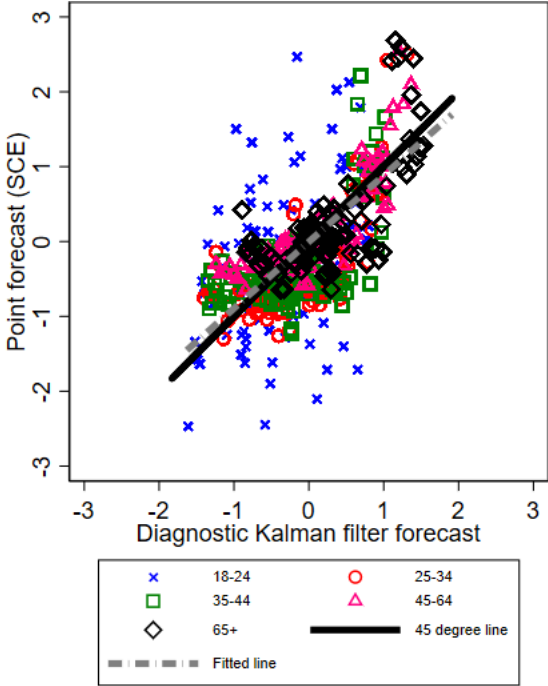
Figure 5: Observed inflation forecasts and diagnostic Kalman filter forecasts
