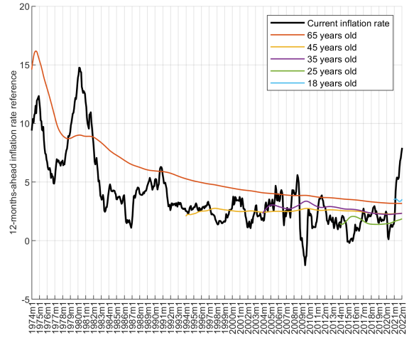
Figure A.6: Diagnostic Kalman-filter-based inflation forecasts by cohort, AR(1)
